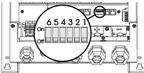
Figure 6. DIP switches
