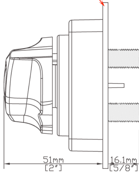
Shallow Intrusion Mounting option
